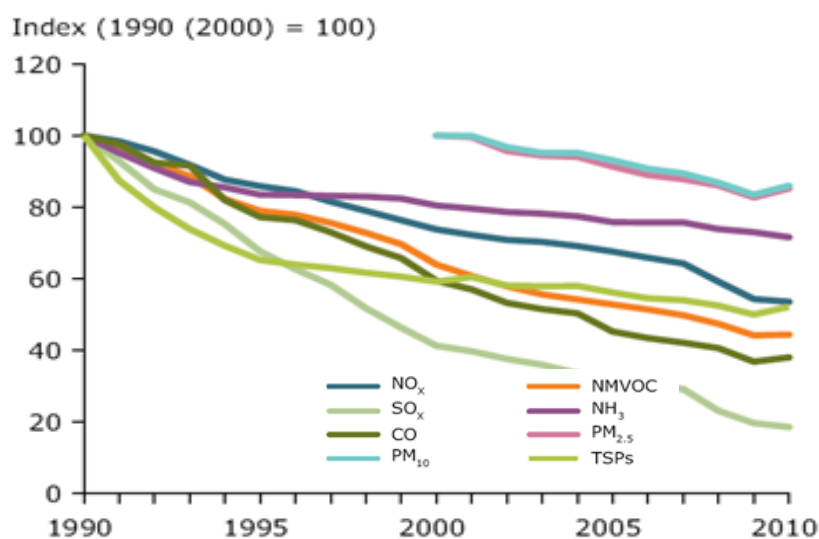
Figure 1: EU air pollutant emissions 1990-2010 (EEA, 2012)
