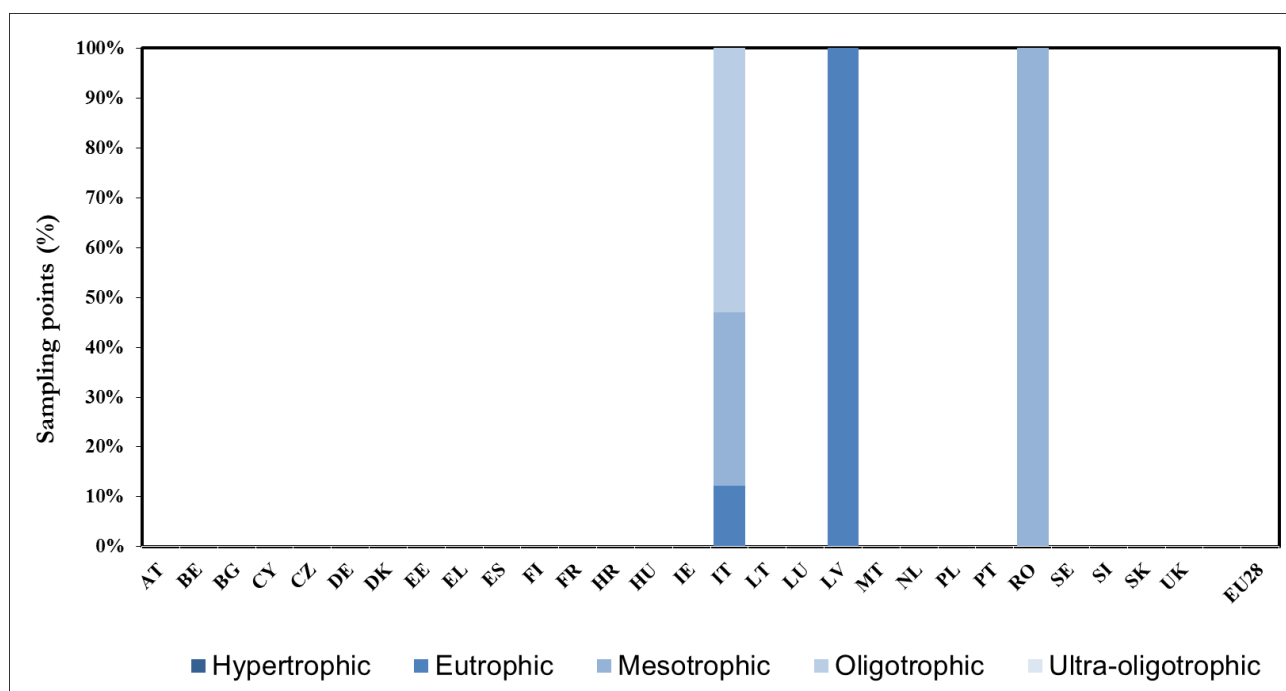
Figure 15. Frequency diagram of trophic status classes of coastal waters in reporting period 2012-2015.
