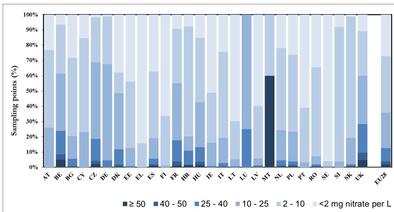
Figure 9. Frequency diagram of annual average nitrate concentrations in fresh surface waters (rivers and lakes).
