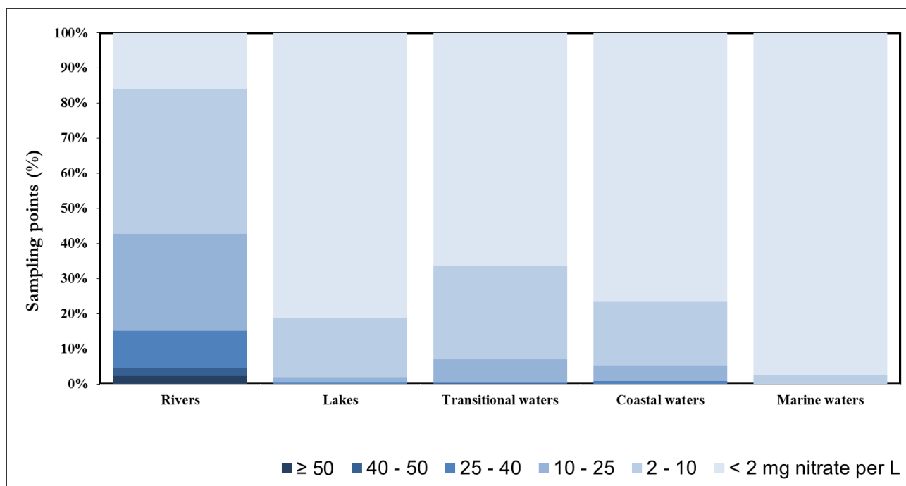
Figure 10. Frequency diagram of annual average nitrate concentrations in different surface waters, aggregated over all Member States.
