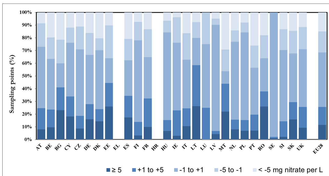
Figure 8. Frequency diagram of trends in annual average nitrate concentrations in groundwater.
