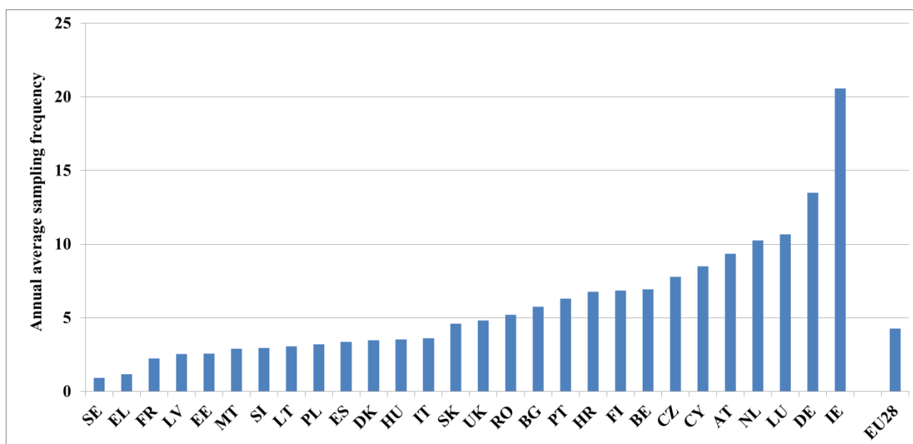
Figure 4. Annual average fresh surface water sampling frequency in reporting period 2012-2015. Stations with data of average annual nitrate measurements.
