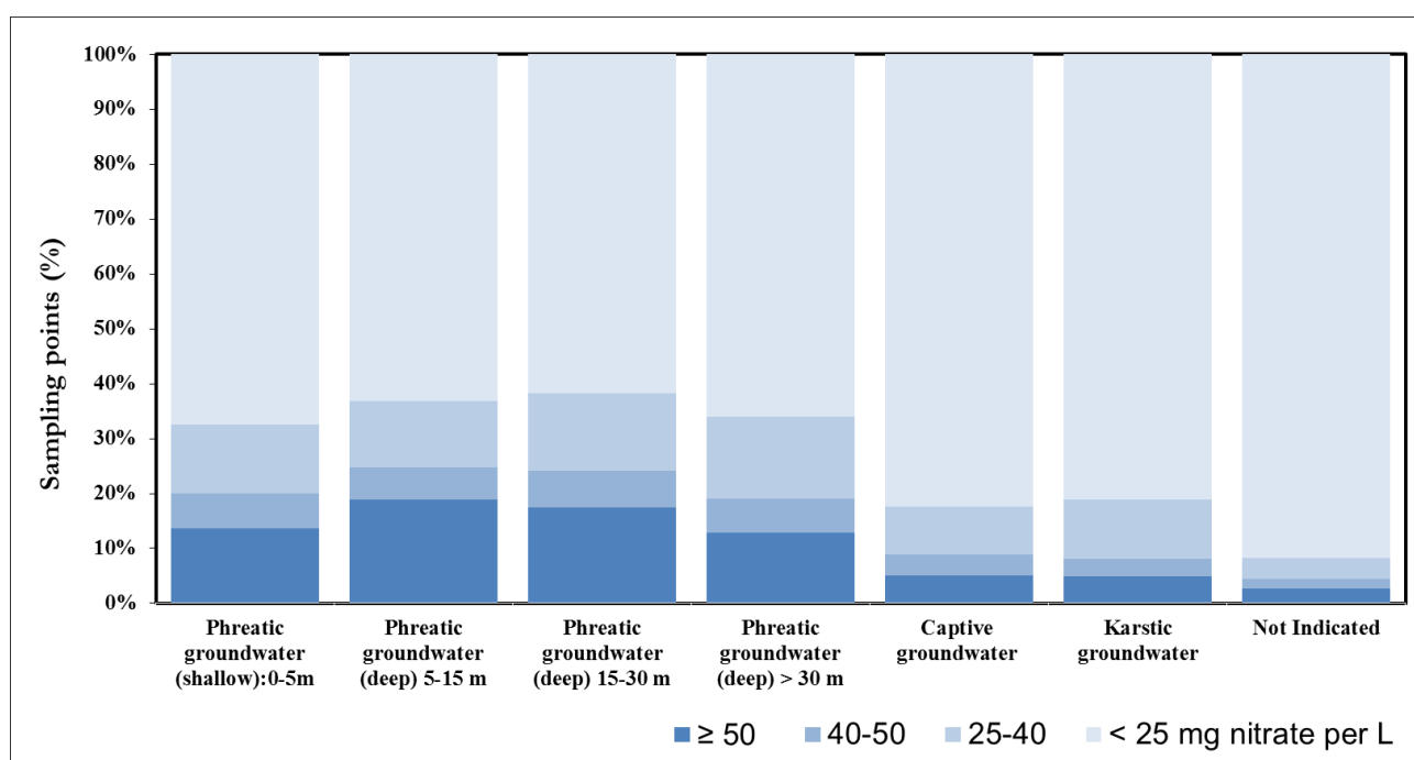
Figure 6. Frequency diagram of annual average nitrate concentrations in groundwater at different depths, aggregated over all Member States.
