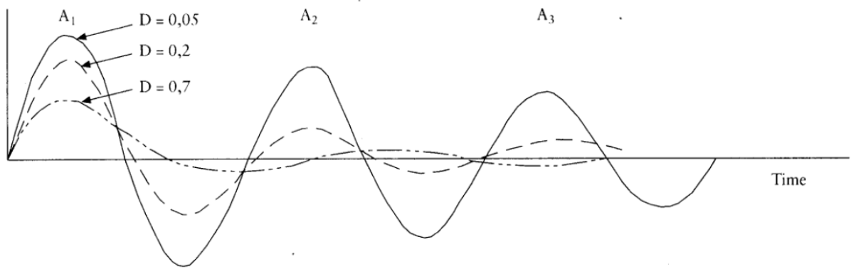
Figure 2 A damped transient response
