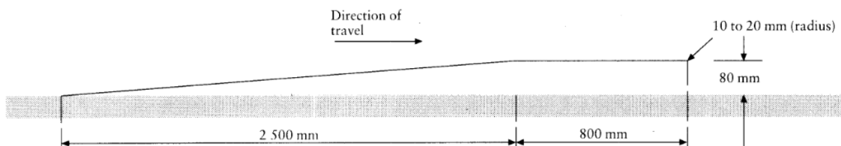
Figure 1 Step for suspension tests
