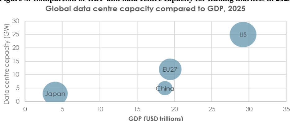
Figure 3. Comparison of GDP and data centre capacity for leading markets in 2025
