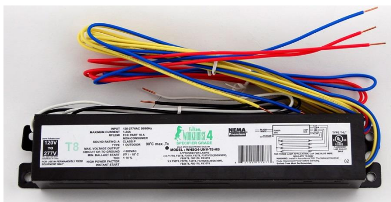
Figure 1: Lighting technologies 5 (above) and example of a control gear for linear fluorescent lamps (below)
