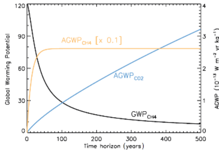
Figure 4. Development of AGWP-CO 2 , AGWP-CH 4 and GWP-CH 4 with time horizon. The yellow and blue curves show how the AGWPs changes with increasing time horizon. Because of the integrative nature the AGWP for CH 4 (yellow curve) reaches a constant level after about five decades. The AGWP for CO 2 continues to increase for centuries. Thus, the ratio which is the GWP (black curve) falls with increasing time horizon (taken directly from Figure 8.29 of Myhre et al., 2013).
