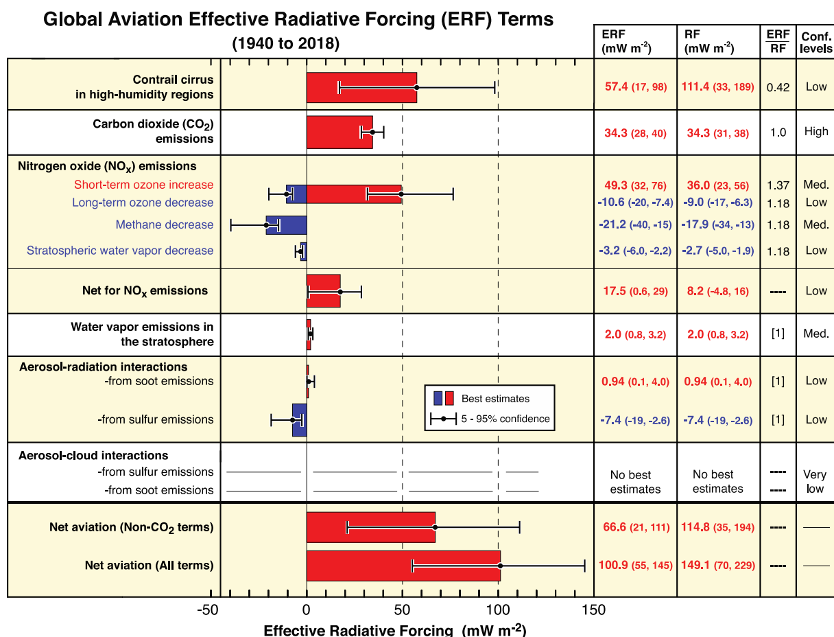
Figure 2. Best-estimates for climate forcing terms from global aviation from 1940 to 2018. The bars and whiskers show ERF best estimates 19 and the 5–95% confidence intervals, respectively. Red bars indicate warming terms and blue bars indicate cooling terms. Numerical ERF and RF values are given in the columns with 5–95% confidence intervals along with ERF/RF ratios and confidence levels. RF values are multiplied by the respective ERF/RF ratio to yield ERF values. ERF/RF values designated as [1] indicate that no estimate is available yet.. Taken from Lee et al. (2020).
