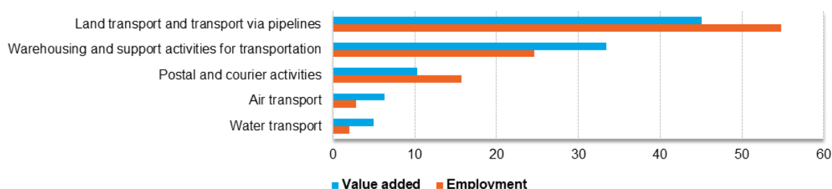
Figure 83: Sectoral analysis of transportation and storage value added and employment in the EU-27 in 2017 (% share of sectoral total)
