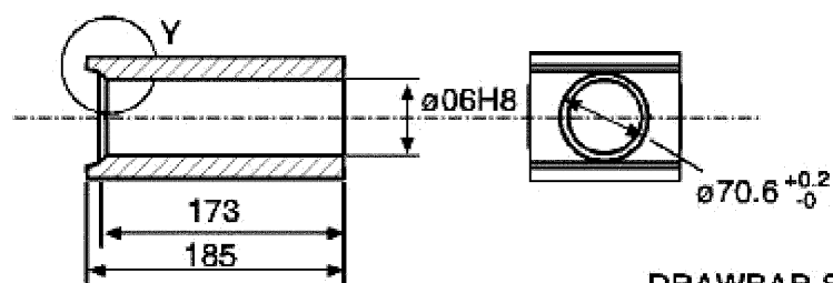
DRAWBAR SOCKET
