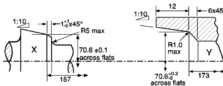
DRAWBAR SOCKET
