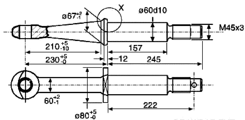
DRAWBAR EYE
