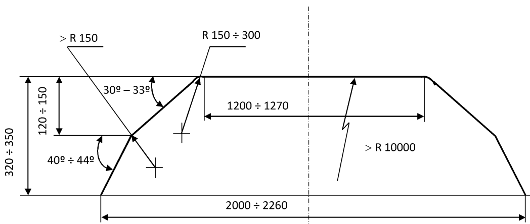
Fig. Configuration and dimensions of contact skates
