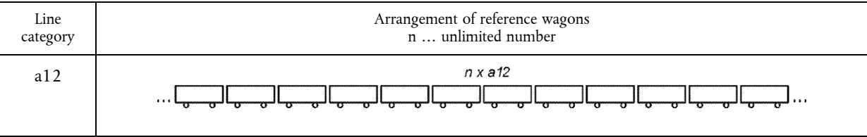
Load model of EN line category a12
