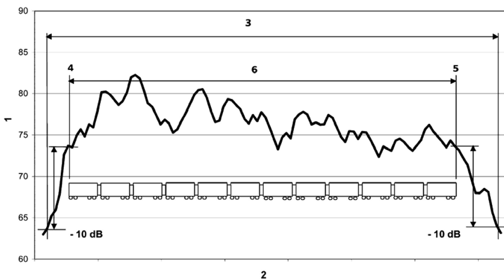
Example of selection of recording time interval, T_{rec} , for a fixed train formation
