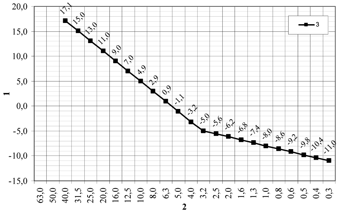
Upper limit curve for the acoustic rail roughness
