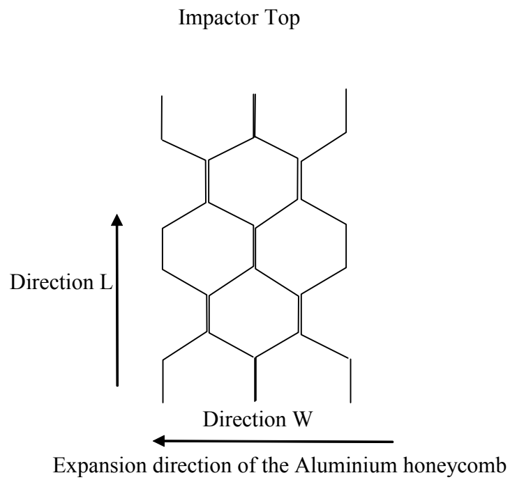
Figure 3 - Aluminium Honeycomb Orientation
