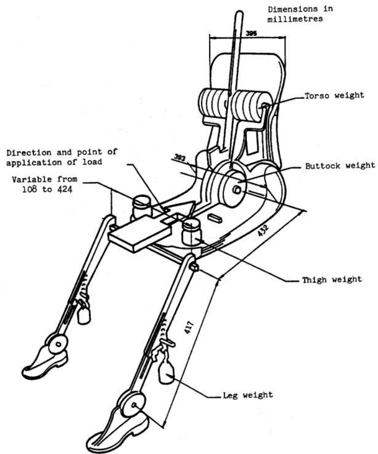
Dimensions of the 3-D H machine elements and load distribution
