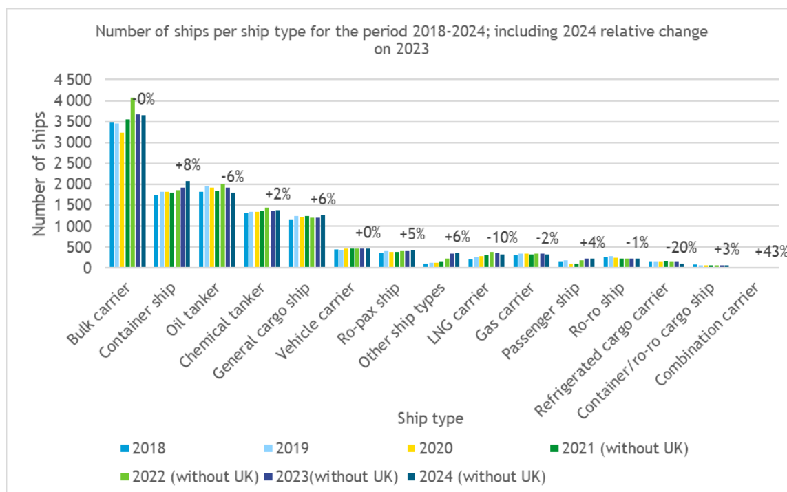
Figure 11: Number of ships per ship type; 2018 to 2024; descending 2024 order; percentage change in 2024 compared to 2023
