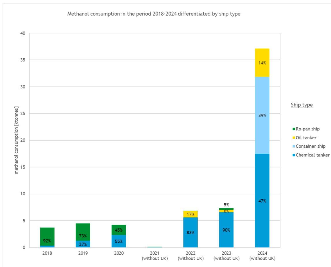
Figure 21: Methanol consumption per ship type 49
