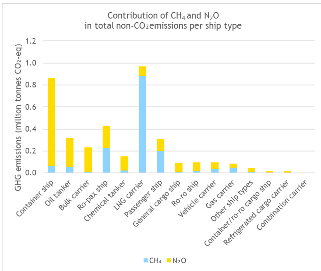
Figure 14: Contribution of CH 4 and N 2 O in total non-CO 2 emissions per ship type
