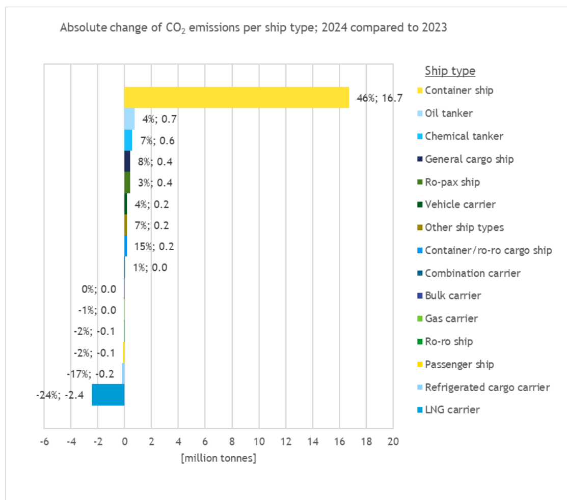
Figure 7: Change of emissions in 2024 compared to 2023 per ship type, in absolute and relative terms
