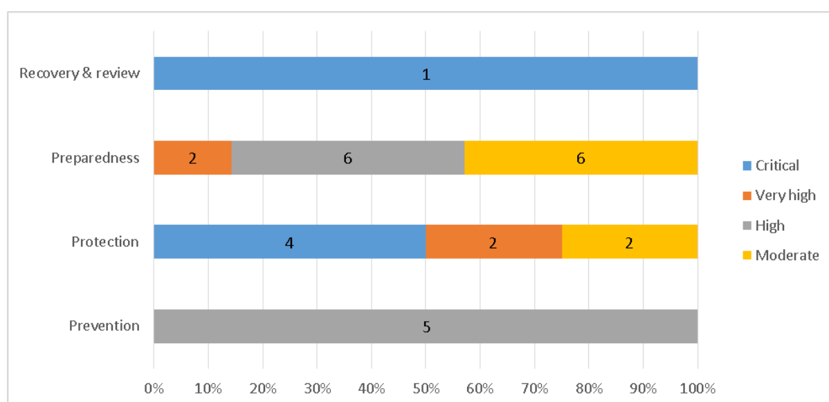
Figure A3 Visualisation of Table A4: Category of priority by measure aspect
