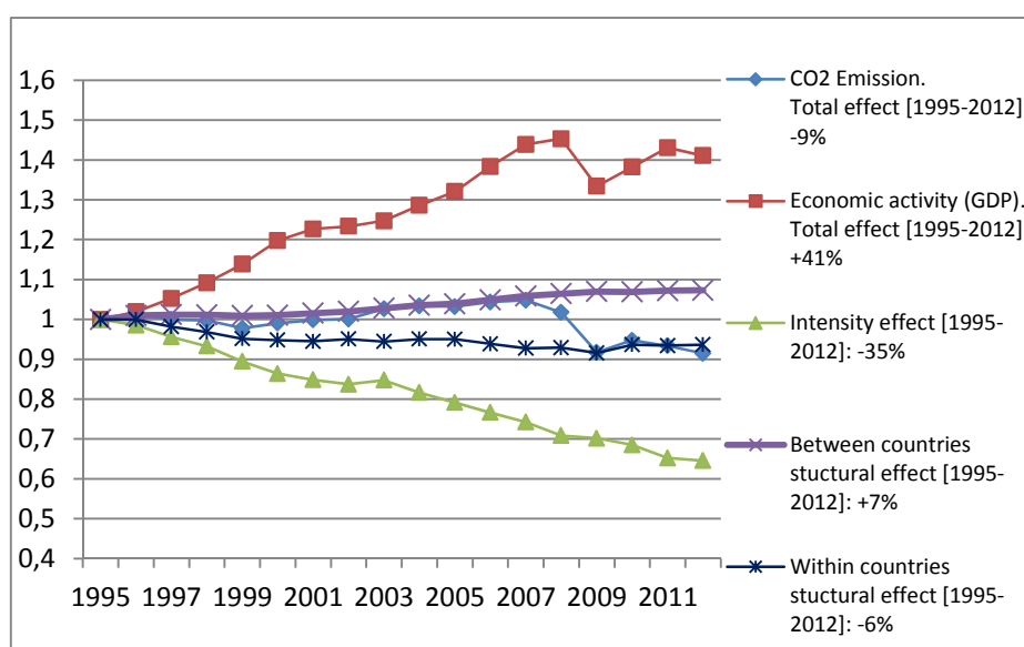
Figure 8: 1995-2012 CO 2 decomposition analysis
