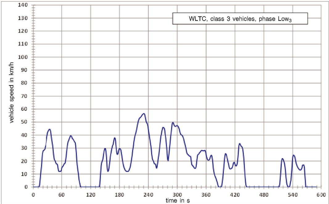
WLTC, Class 3 vehicles, phase Low 3
