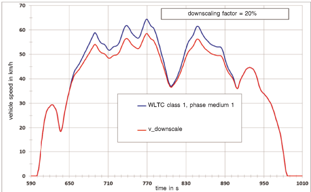
Downscaled medium speed phase of the class 1 WLTC
