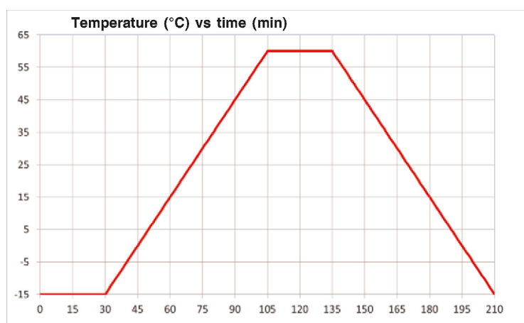
Temperature conditioning cycle
