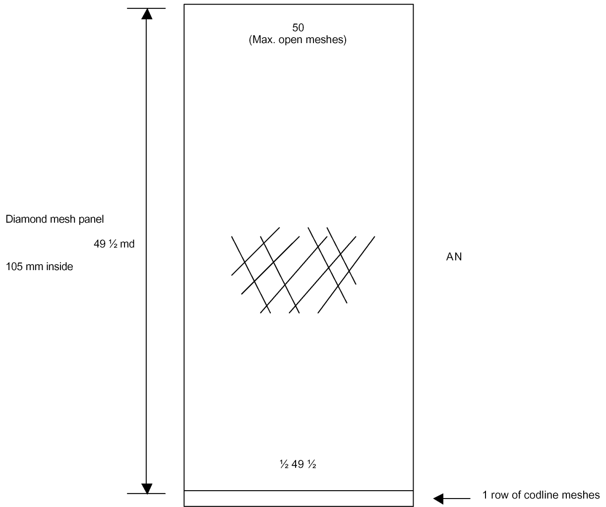
Showing the construction of lower panel made of 49,5 meshes deep netting
