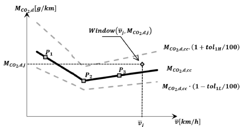
Vehicle CO 2 characteristic curve and tolerances for ICE and NOVC-HEV vehicles
