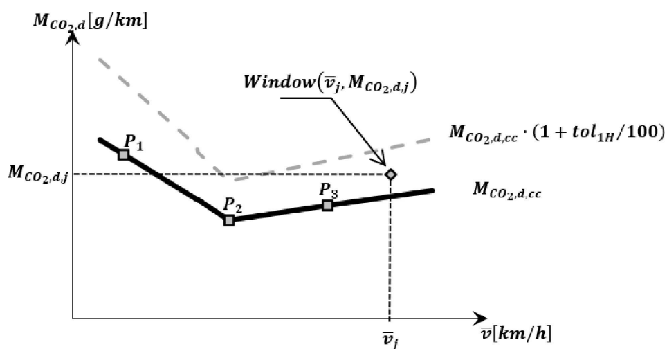
Vehicle CO 2 characteristic curve and tolerances for OVC-HEV vehicles
