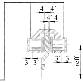
disk brake
