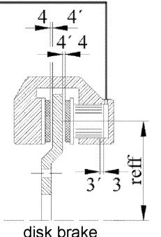
disk brake
