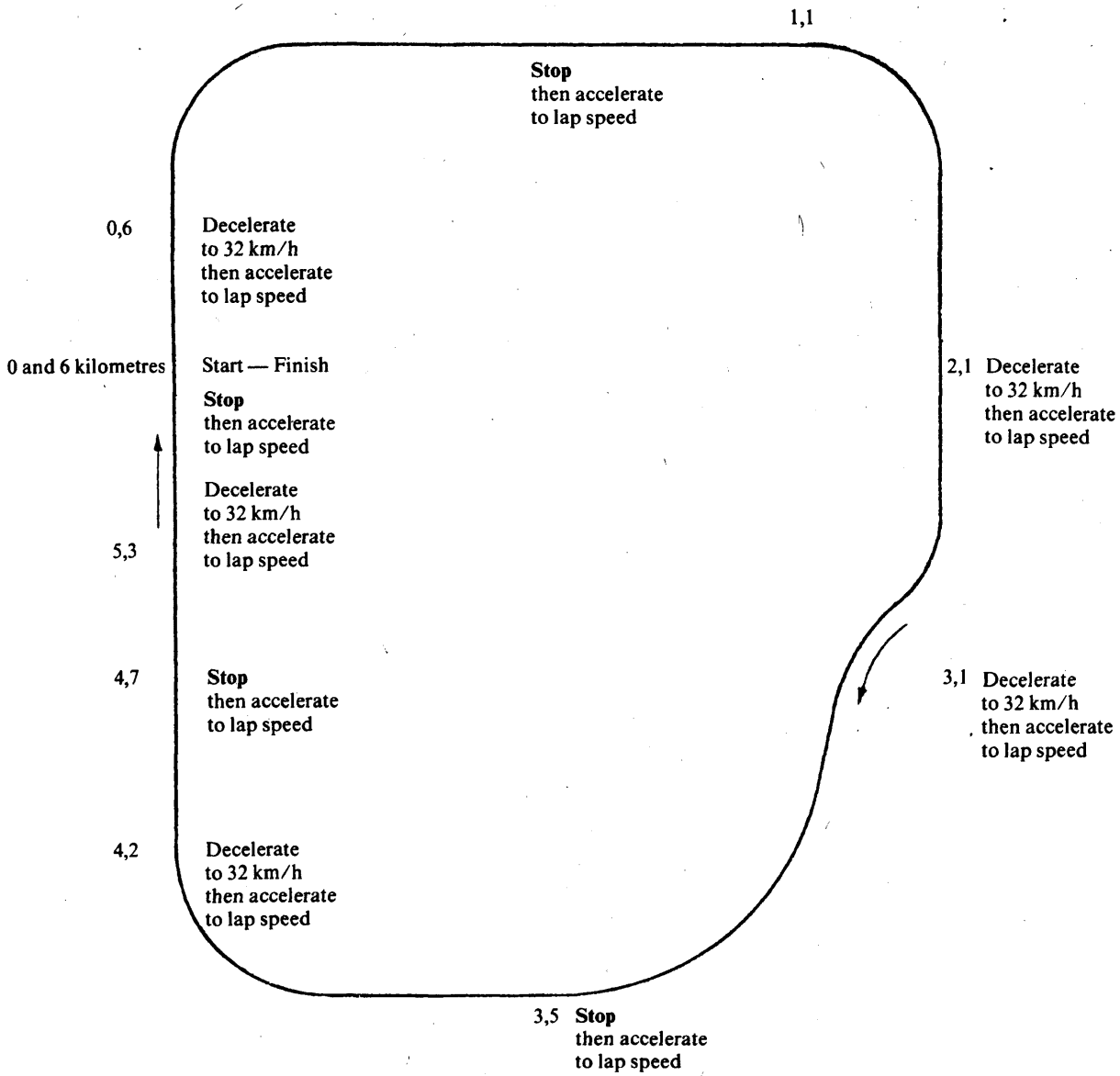
Figure VII.5.1 Driving schedule
