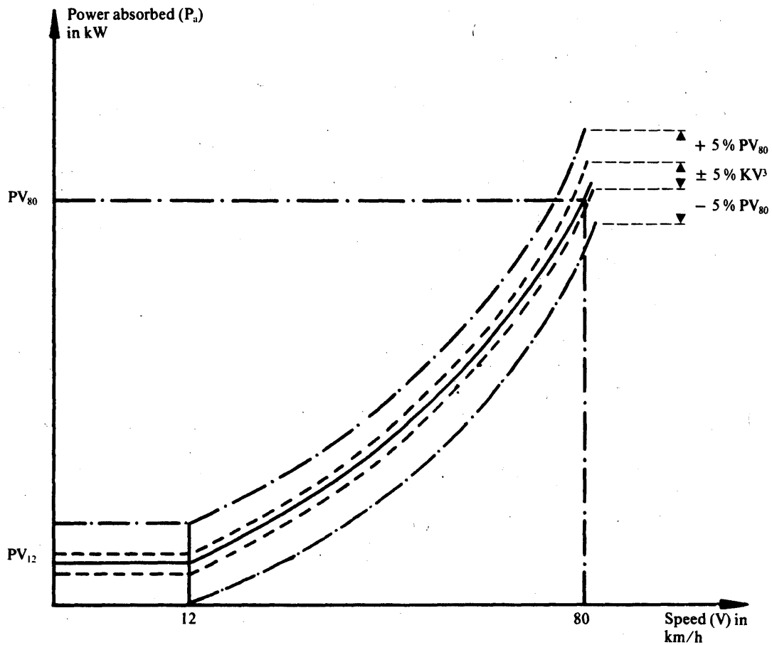
Diagram illustrating the power of the chassis dynamometer
