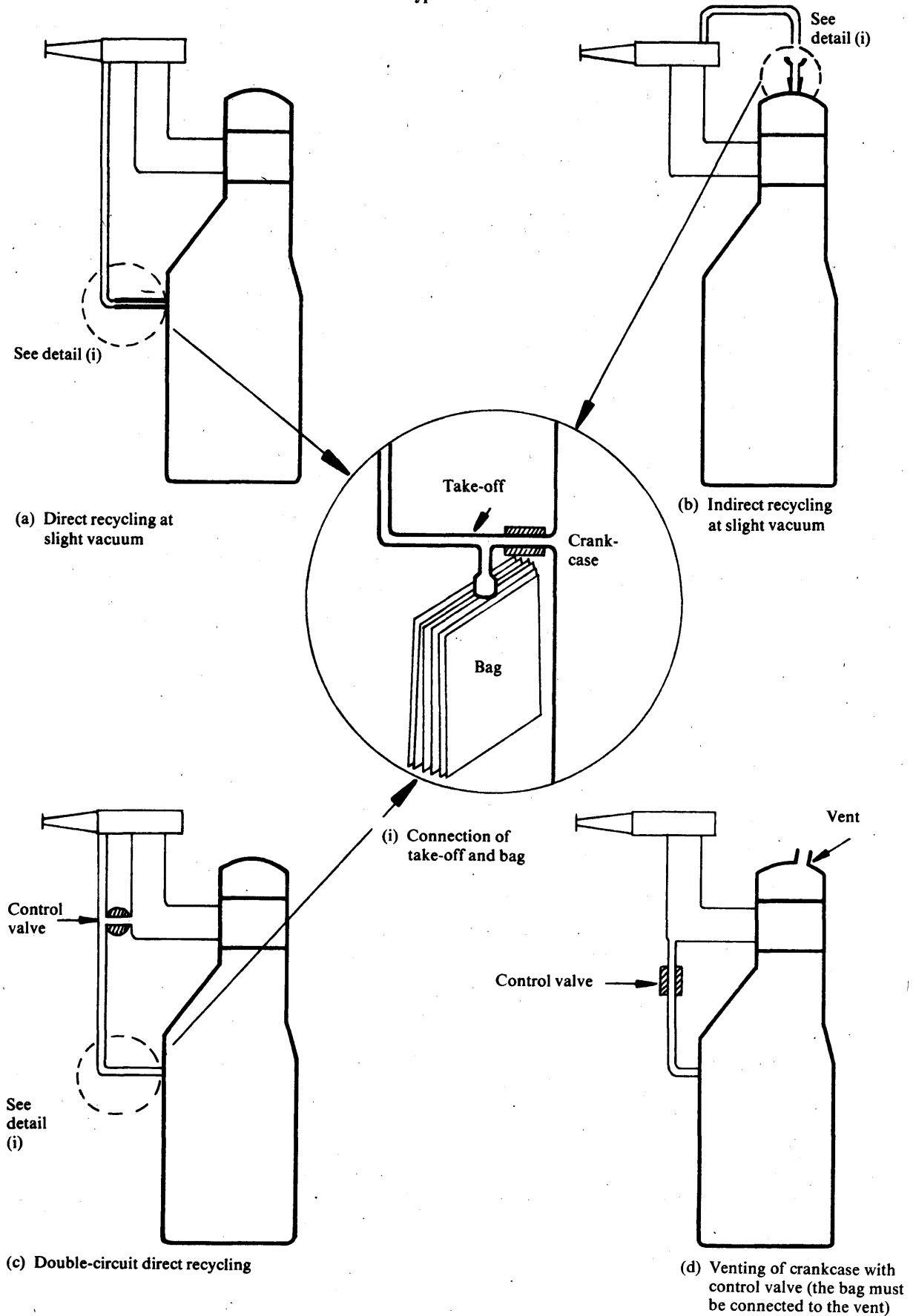
Figure V.5. Type III test
