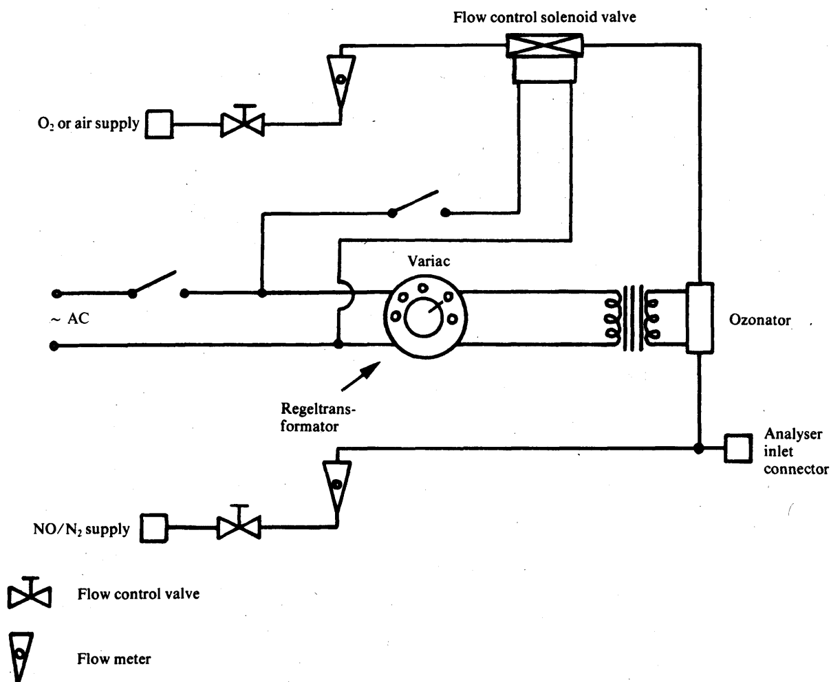
Diagram of NO x converter efficiency device
