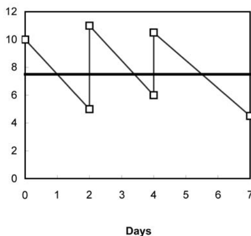
Figure 1: Example of time-weighted mean
