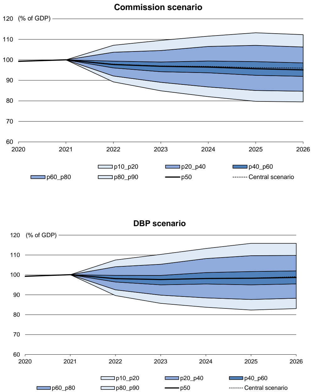
Graph III.1: Fan charts from stochastic public debt projections around the Commission's forecast scenario and the Draft Budgetary Plans' forecast scenario; euro area
