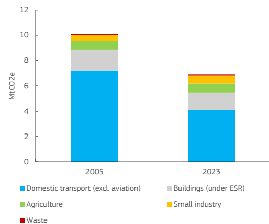
Graph A7.2: Greenhouse gas emissions from the effort sharing sectors, 2005 and 2023
