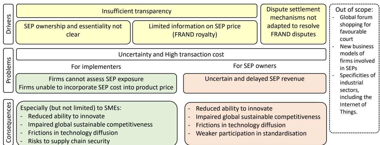
Figure 3: Problem tree
