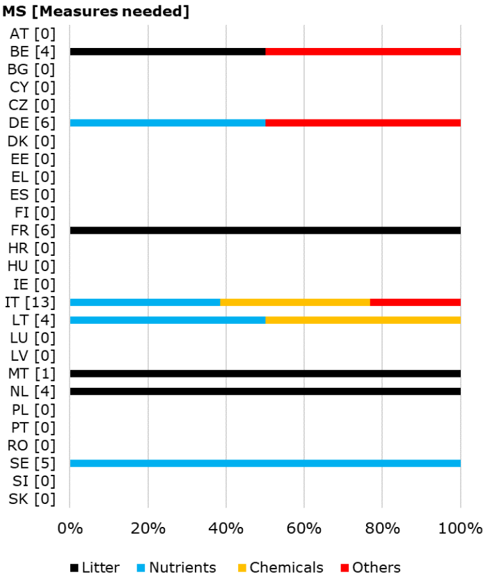
Figure 22: Member State reporting the types of additional measures needed to meet the MSFD objectives.
