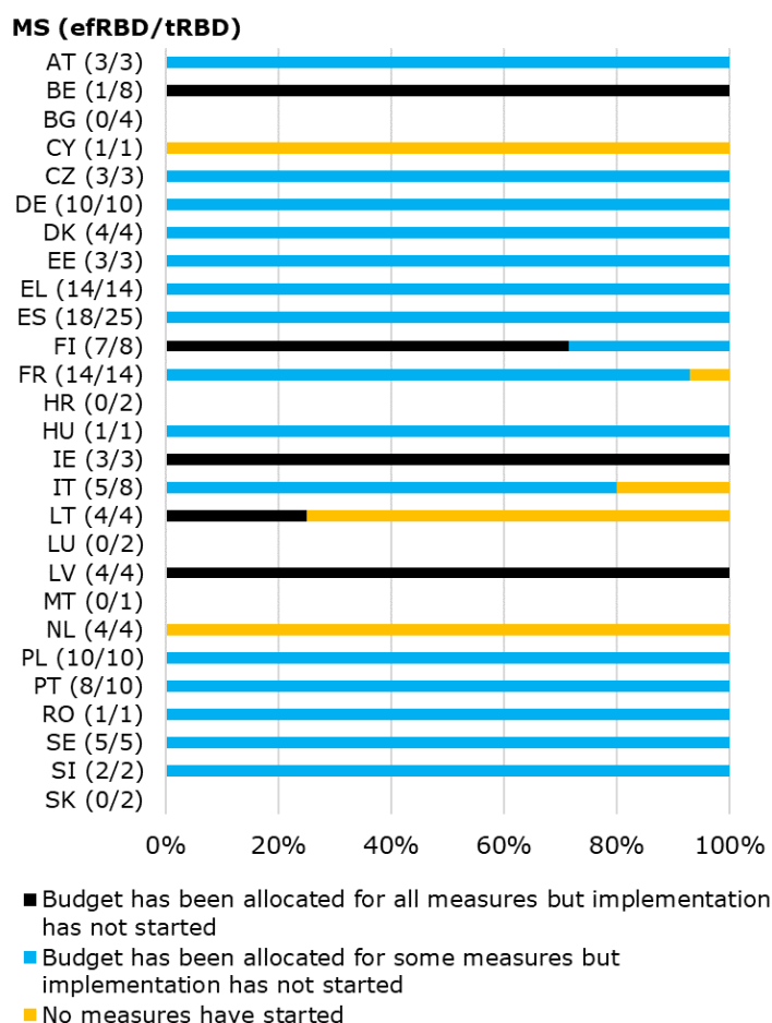
Figure 18: Member State reporting on whether budgets for ecological flows have been allocated. efRBD = RBD where ecological flows have been derived fully or partly. trRBD = total number of RBDs.
