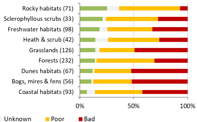
Figure 4b: Conservation status per habitat group at EU level
