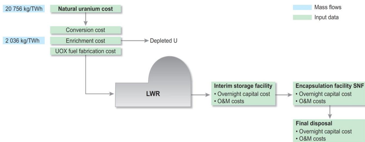
Figure 20 Illustrative once-through (OT) cycle 94
