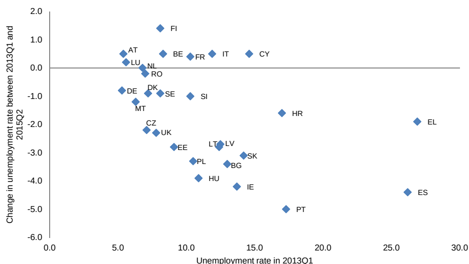
Graph 10: Evolution of the unemployment rate since 2013
