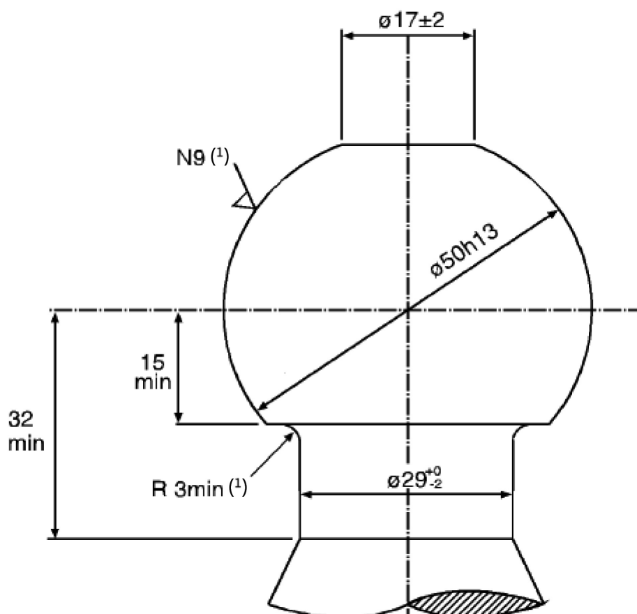
Coupling ball of Class A
