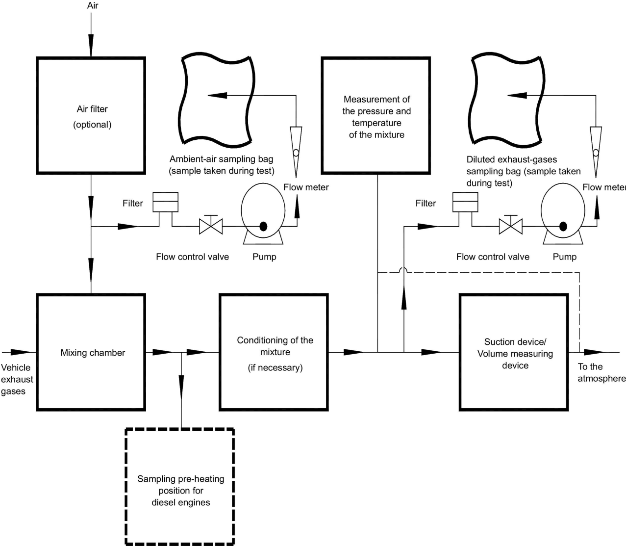
Diagram of a variable-dilution system for measuring exhaust gas emissions
