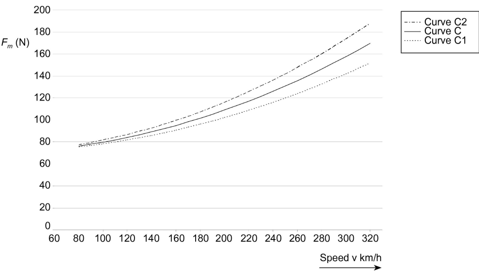
Figure 4.2.15.1 Mean contact force F_m for AC systems as a function of speed
