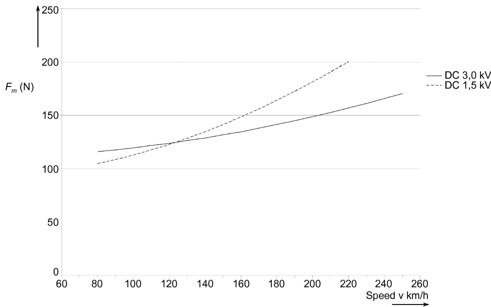
Figure 4.2.15.2 Mean contact force F_m for DC systems as a function of speed
