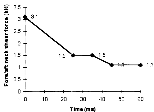
Figure 2 Neck Shear Criterion
