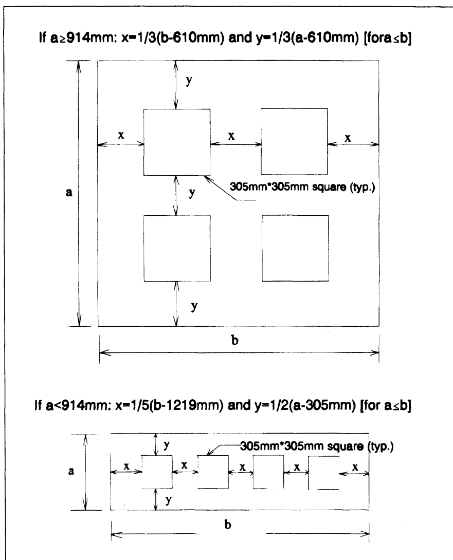
Figure 2 – Locations of Samples for Certification
