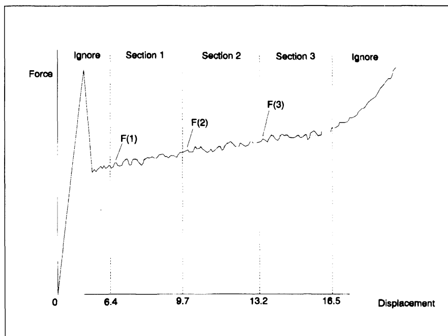
Figure 4 — Crush Force and Displacement
