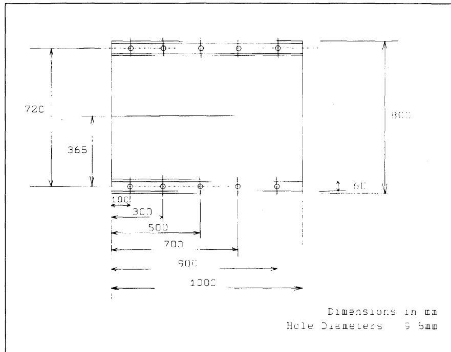
Figure 5 — Positions of Holes for Barrier Mounting
