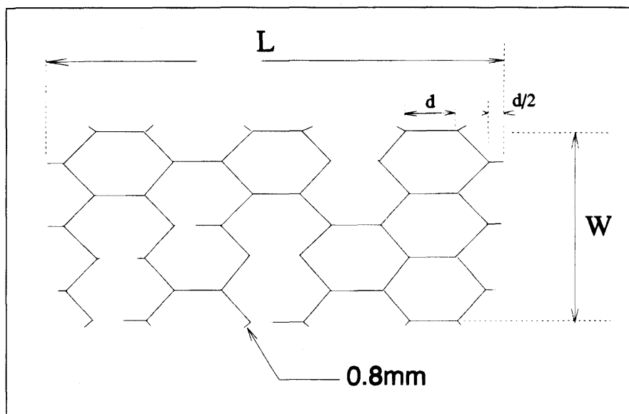
Figure 3 — Honeycomb Axes and Measured Dimensions
