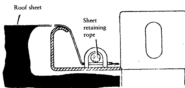
Sectional view
