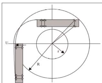
Figure 2a: rear swing-out (non-articulated vehicles)
