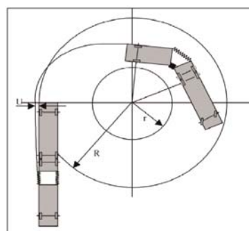
Figure 2b: rear swing-out (articulated vehicles)
