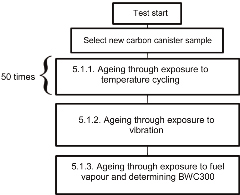
Figure C3/1 Carbon canister bench ageing procedure
