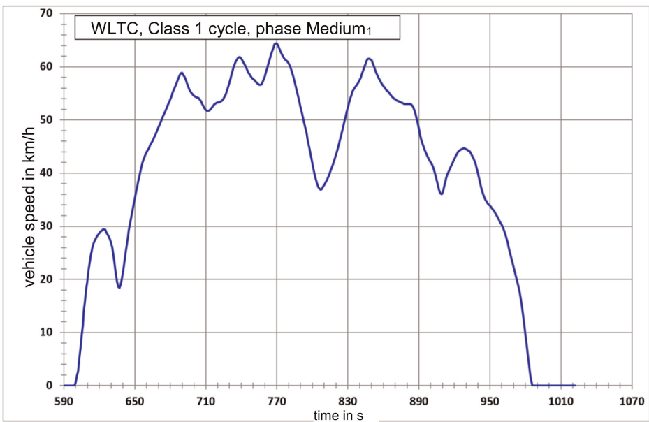
WLTC, Class 1 cycle, phase Medium 1
