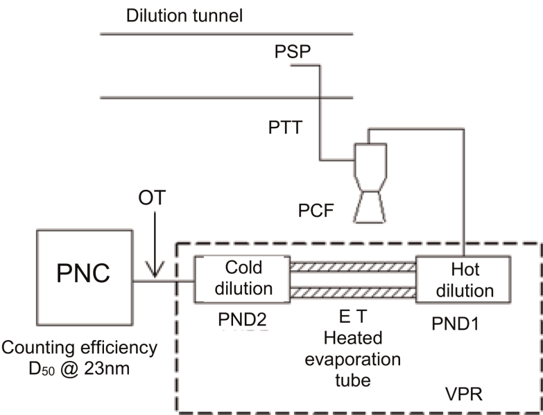
Figure A5/14 A recommended particle sampling system
