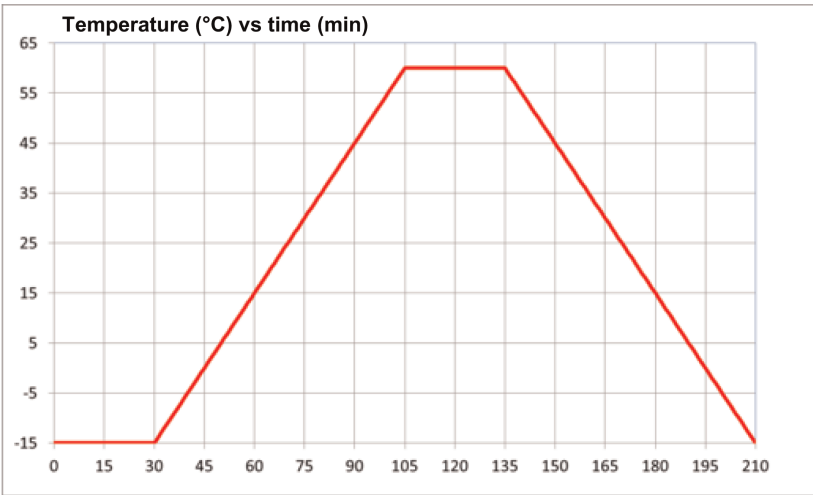
Figure C3/2 Temperature conditioning cycle
