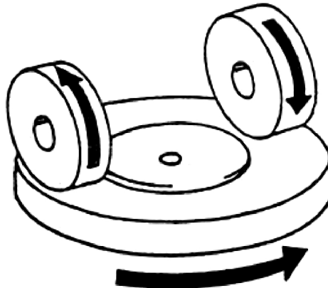
Figure 4 — Diagram of abrading instrument
