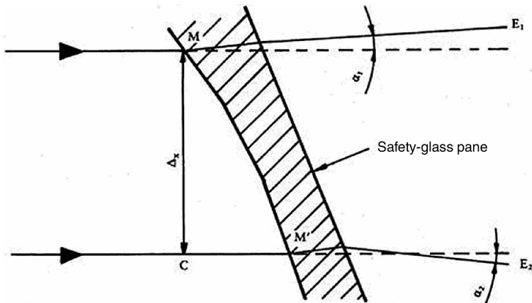
Figure 6 — Diagrammatic representation of optical distortion
