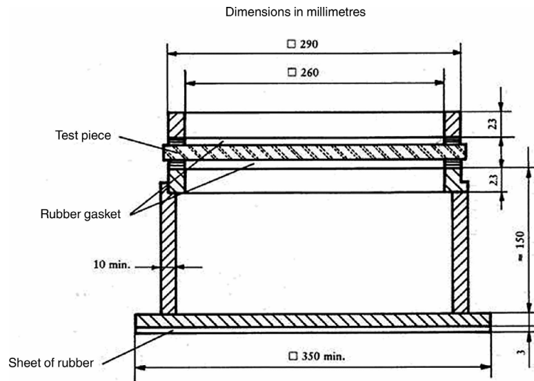
Figure 1 — Support for ball tests
