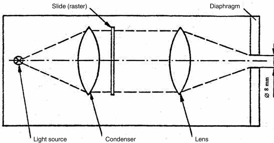
Figure 7 — Optical arrangement of the projector
