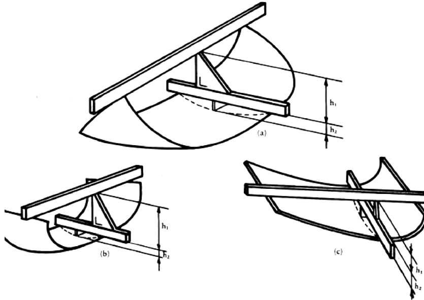
Figure 1 — Determination of height of segment, h
