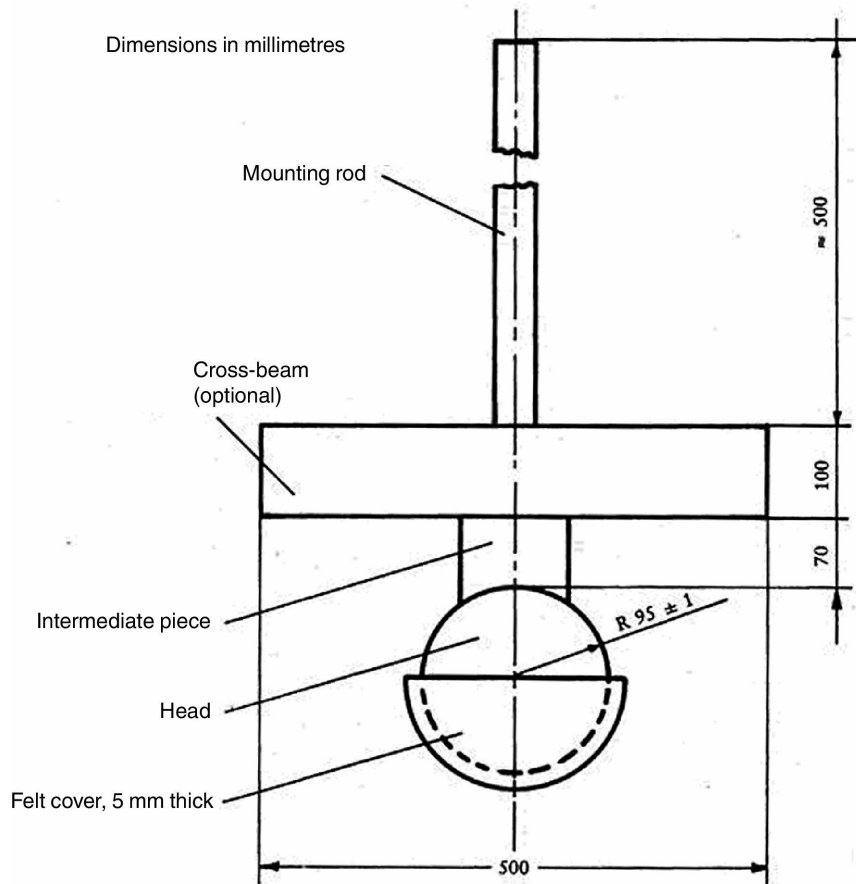
Figure 2 — Headform weight
