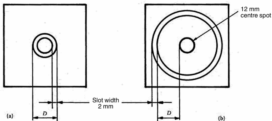
Figure 11 — Dimensions of targets
