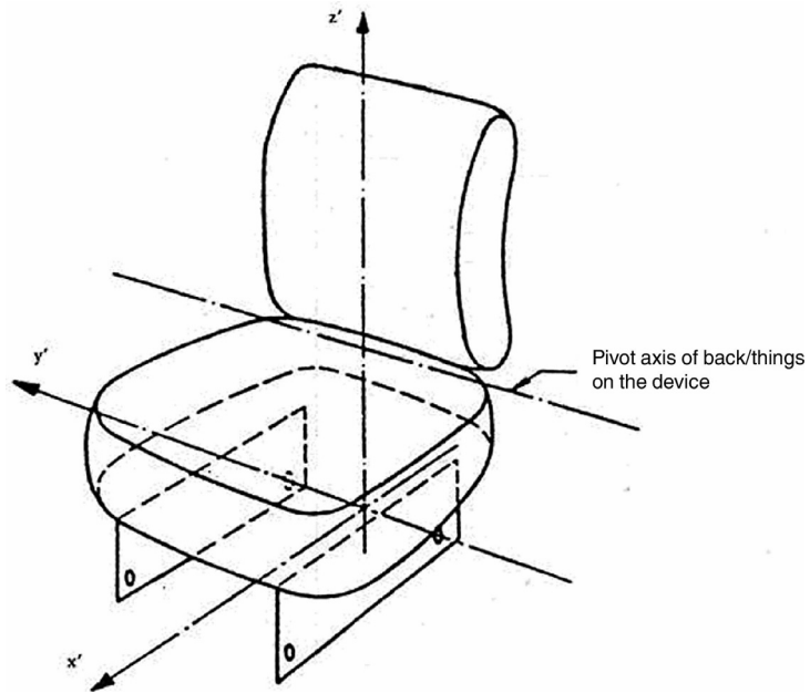
Figure 11 — Determination of SIP reference axes
