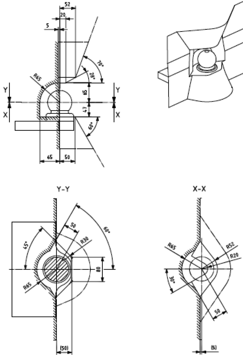
Ball type coupling (corresponding to ISO 24347:2005)
