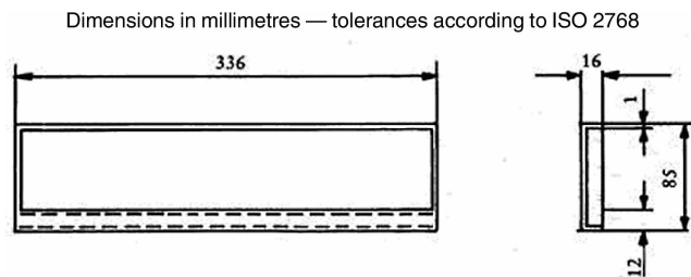
Figure 17 — Typical drip pan
