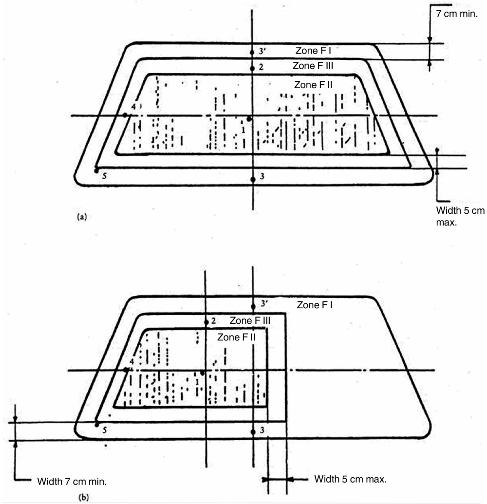
Figure 2 — Prescribed points of impact for windscreens
