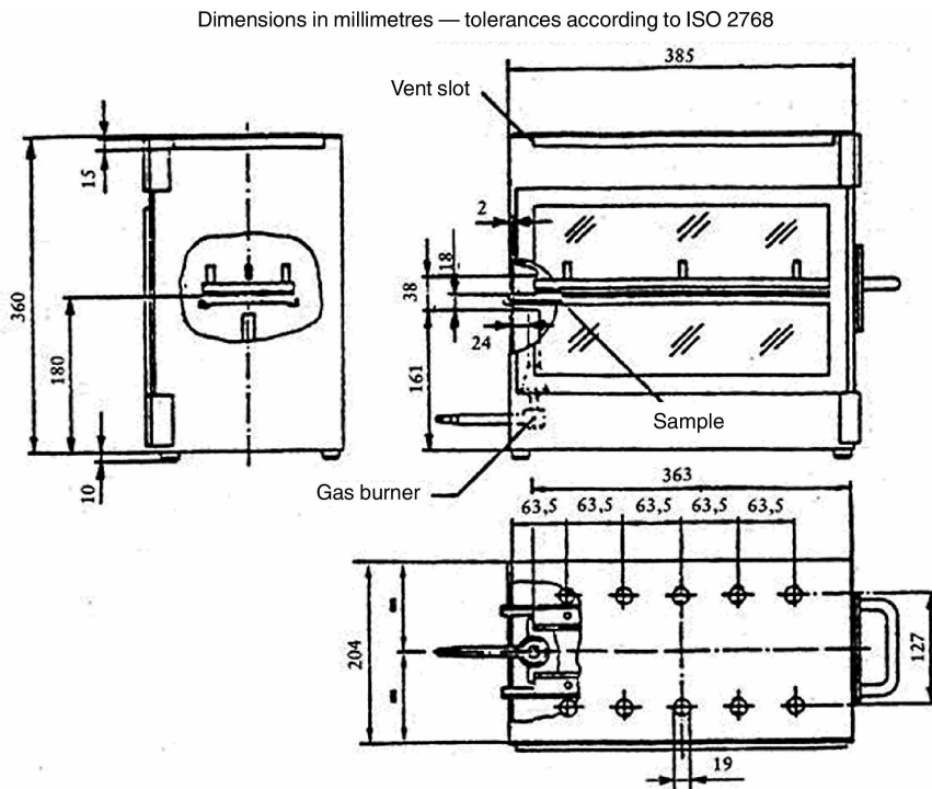
Figure 16 — Example of combustion chamber
