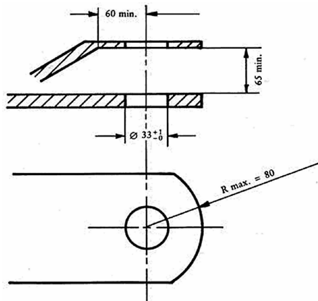
Figure 3 — Tractor drawbar
