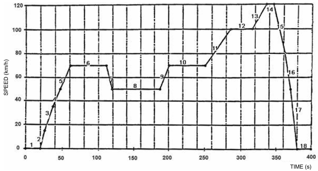
Figure 3 Extra-urban cycle (400 seconds)
