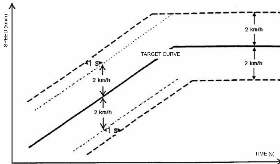
Figure 4 Speed tolerance
