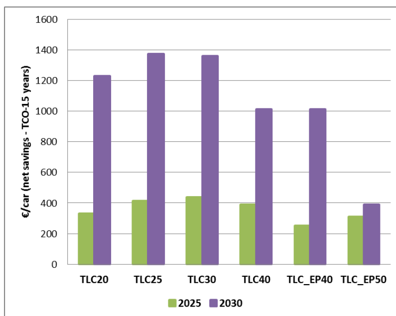
Figure 13: TCO-15 years (vehicle lifetime) (net savings in EUR/car in 2025 and 2030)
