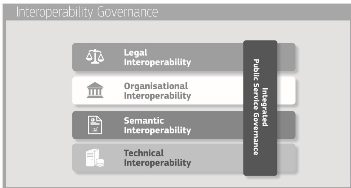
Figure 3: Interoperability model
