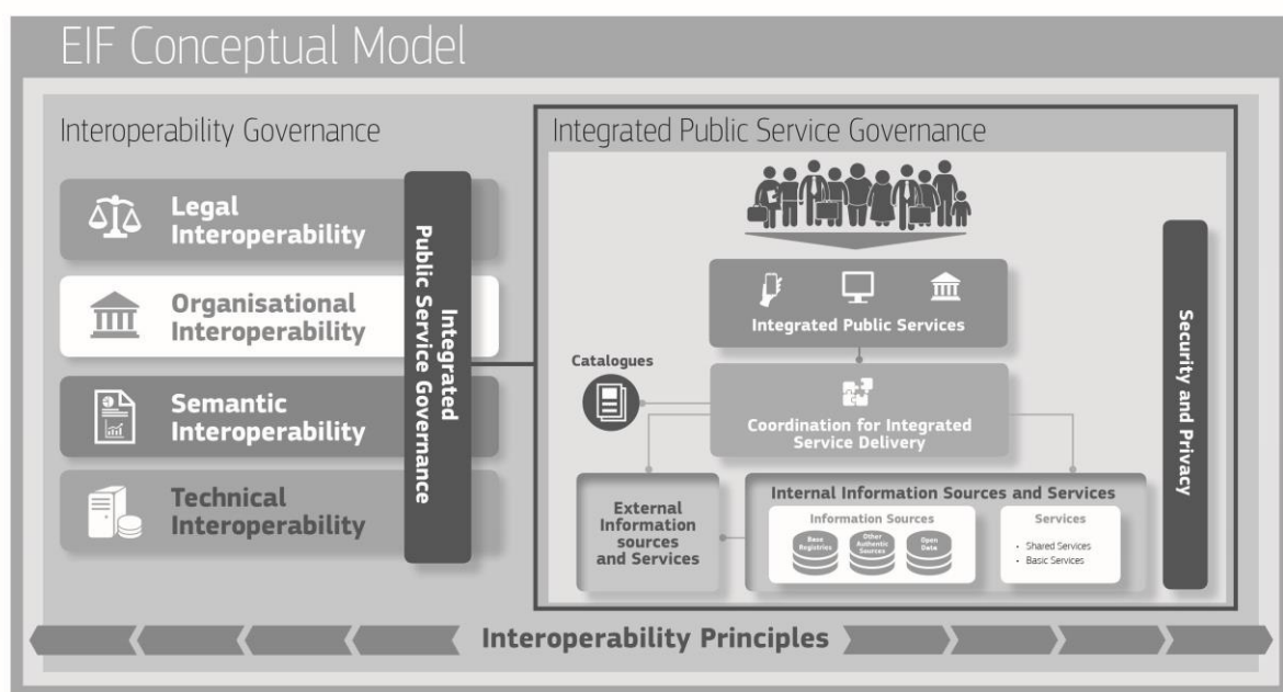
Figure 5: EIF conceptual model relations
