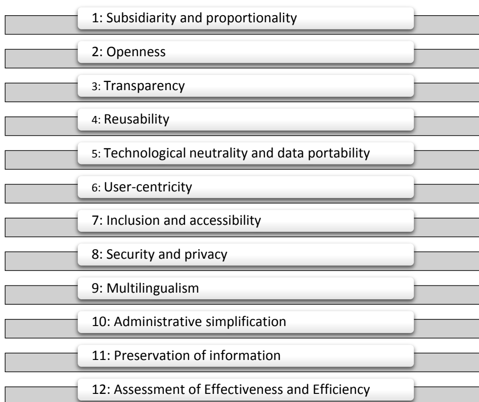
Figure 2: Interoperability principles
