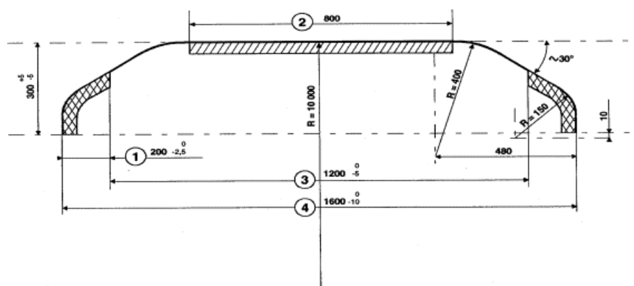
Profile of pantograph head
