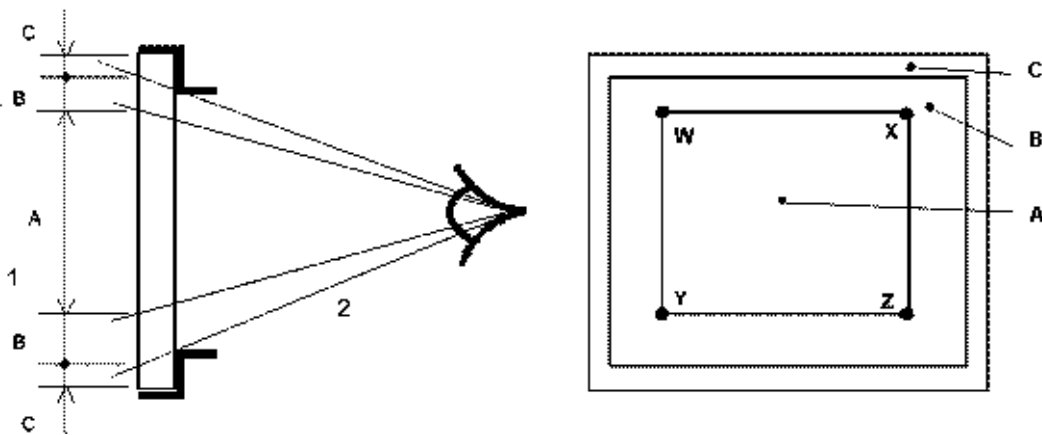
Figure J.1 Windscreen Areas
