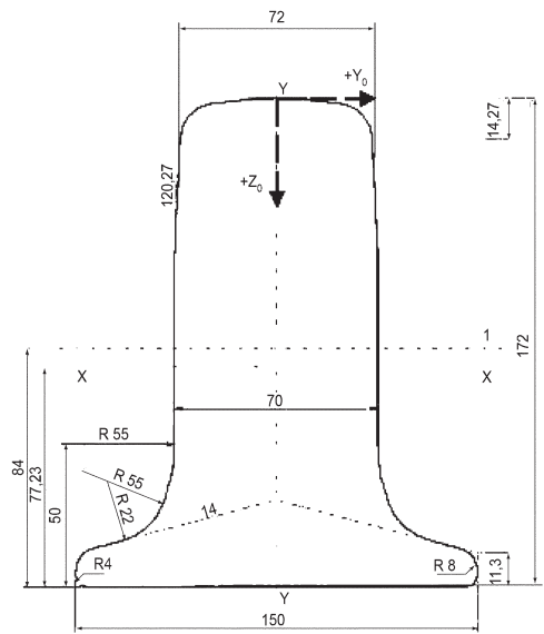
Dimensions in millimeter
