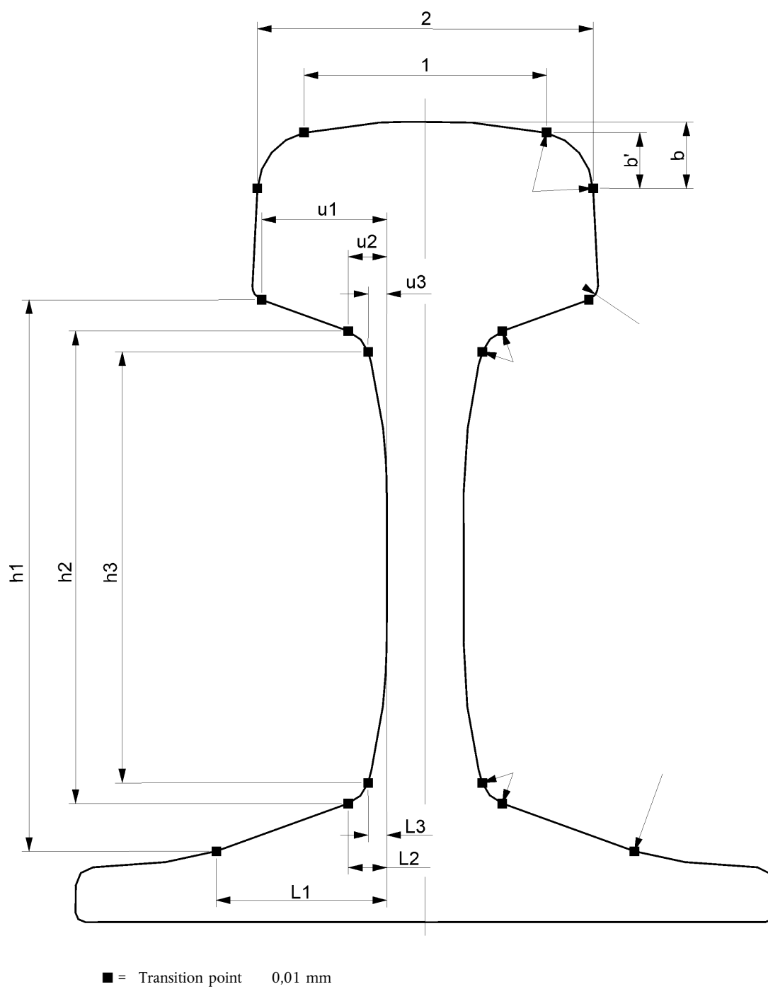
Principal rail transition references
