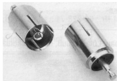
Figure 4 Coaxial socket
