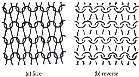
Figure 1 Single jersey (plain knit)
